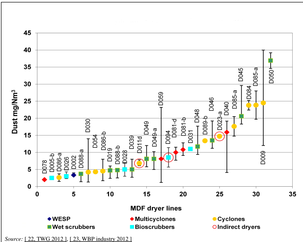
Figure 3.9: Values for dust in emissions to air from MDF dryers and the applied abatement techniques, based on data from 32 production lines
