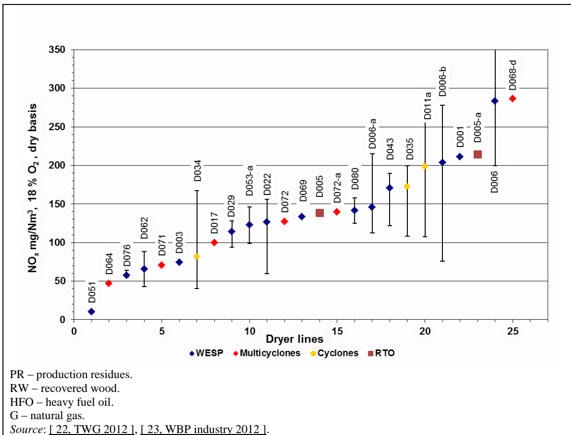
Figure 3.15: NO x emissions to air from directly heated PB dryers with the corresponding emission airflow
