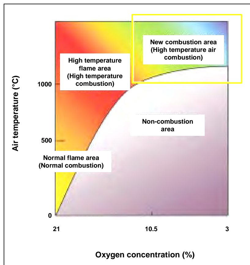
Figure 3.4: Different regions of combustion [17, Åsbländ, 2005]
